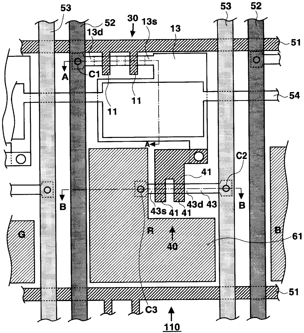
Fig. 2 PRIOR ART
